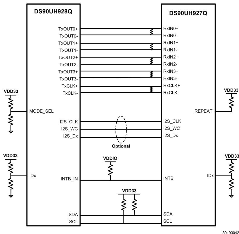
FIGURE 19. HDCP Repeater Connection Diagram
