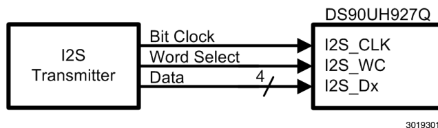
FIGURE 15. I2S Connection Diagram
